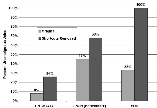
Figure 8: Reducing Ambiguity by Removing Shortcut Joins
