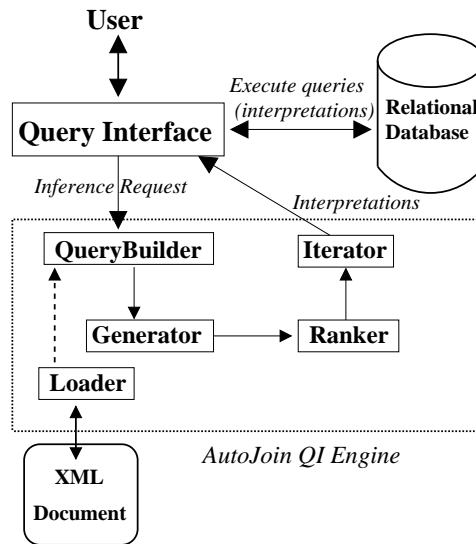
Figure 2: AutoJoin Architecture
