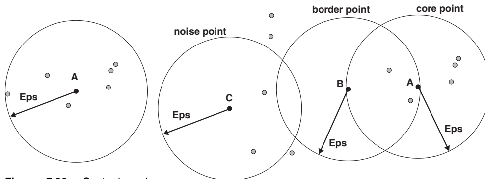
Figure 7.20. Center-based density.
