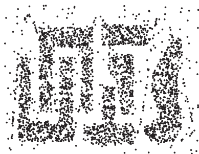
Figure 7.22. Sample data.
