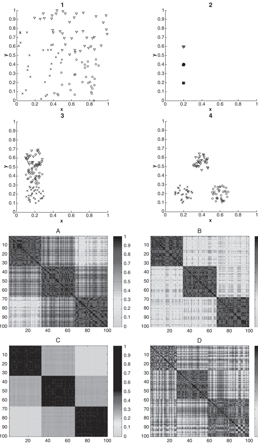
Figure 7.41. Points and similarity matrices for Exercise 32.
