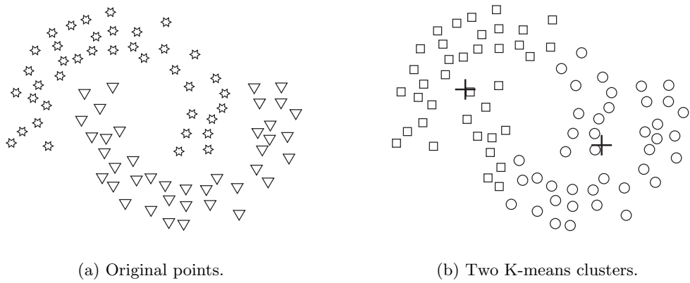
Figure 7.11. K-means with non-globular clusters.
