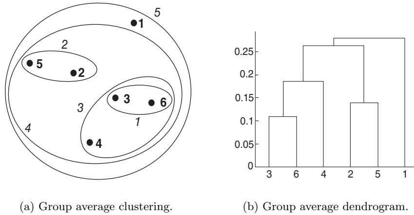
Figure 7.18. Group average clustering of the six points shown in Figure 7.15.
