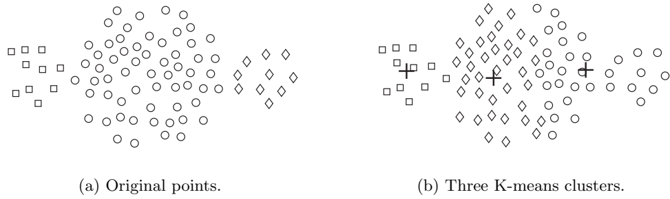
Figure 7.9. K-means with clusters of different size.
