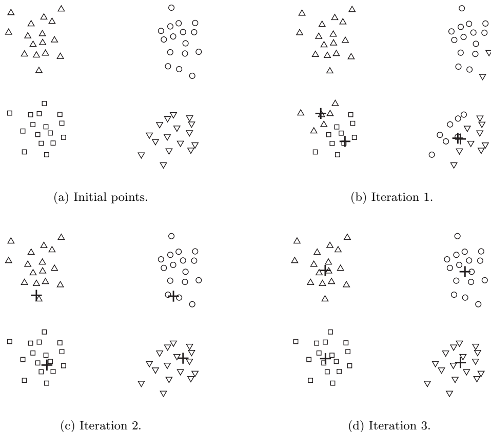
Figure 7.6. Two pairs of clusters with a pair of initial centroids within each pair of clusters.
