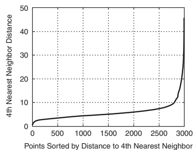
Figure 7.23. K-dist plot for sample data.
