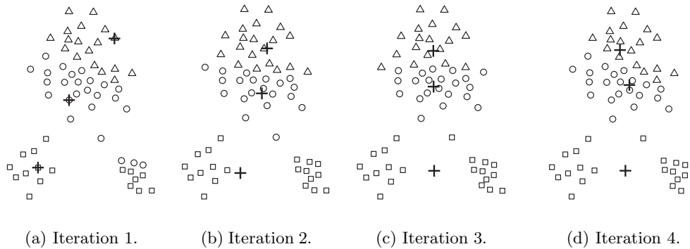
Figure 7.5. Poor starting centroids for K-means.
