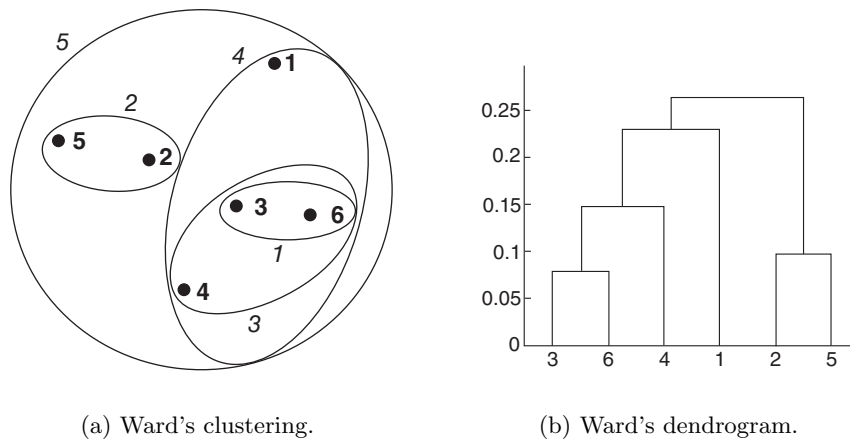
Figure 7.19. Ward's clustering of the six points shown in Figure 7.15.
