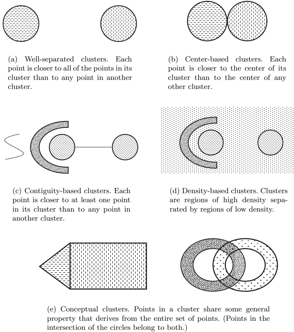
Figure 7.2. Different types of clusters as illustrated by sets of two-dimensional points.
