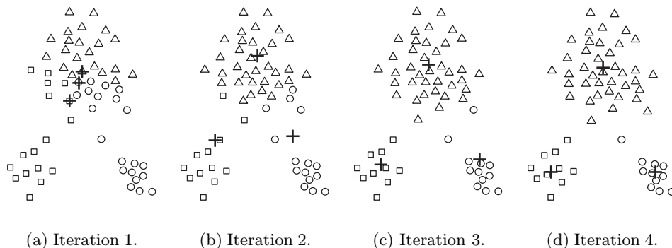
Figure 7.3. Using the K-means algorithm to find three clusters in sample data.
