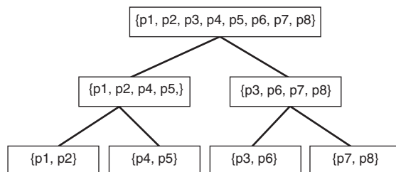
Figure 7.40. Hierarchical clustering for Exercise 25.
