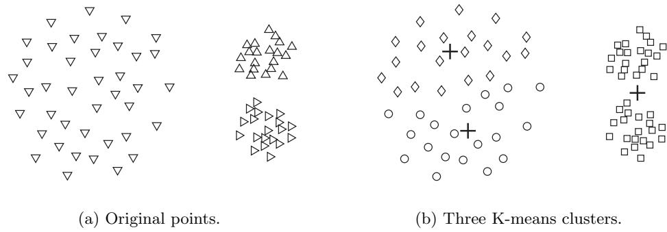
Figure 7.10. K-means with clusters of different density.
