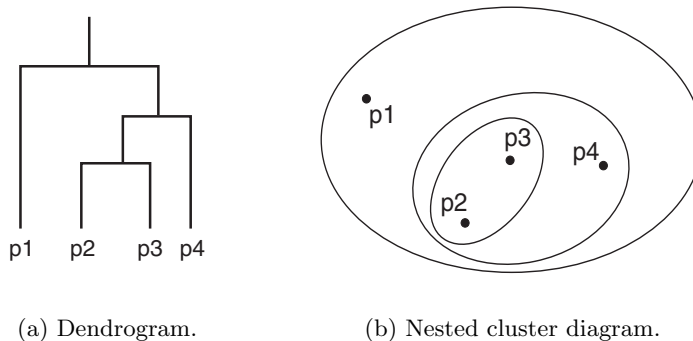
Figure 7.13. A hierarchical clustering of four points shown as a dendrogram and as nested clusters.
