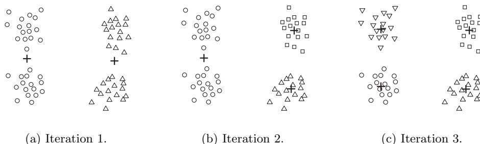
Figure 7.8. Bisecting K-means on the four clusters example.
